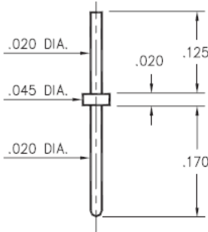
9081-0-00-XX-00-00-08-0 Solder mount in .024 mounting hole
